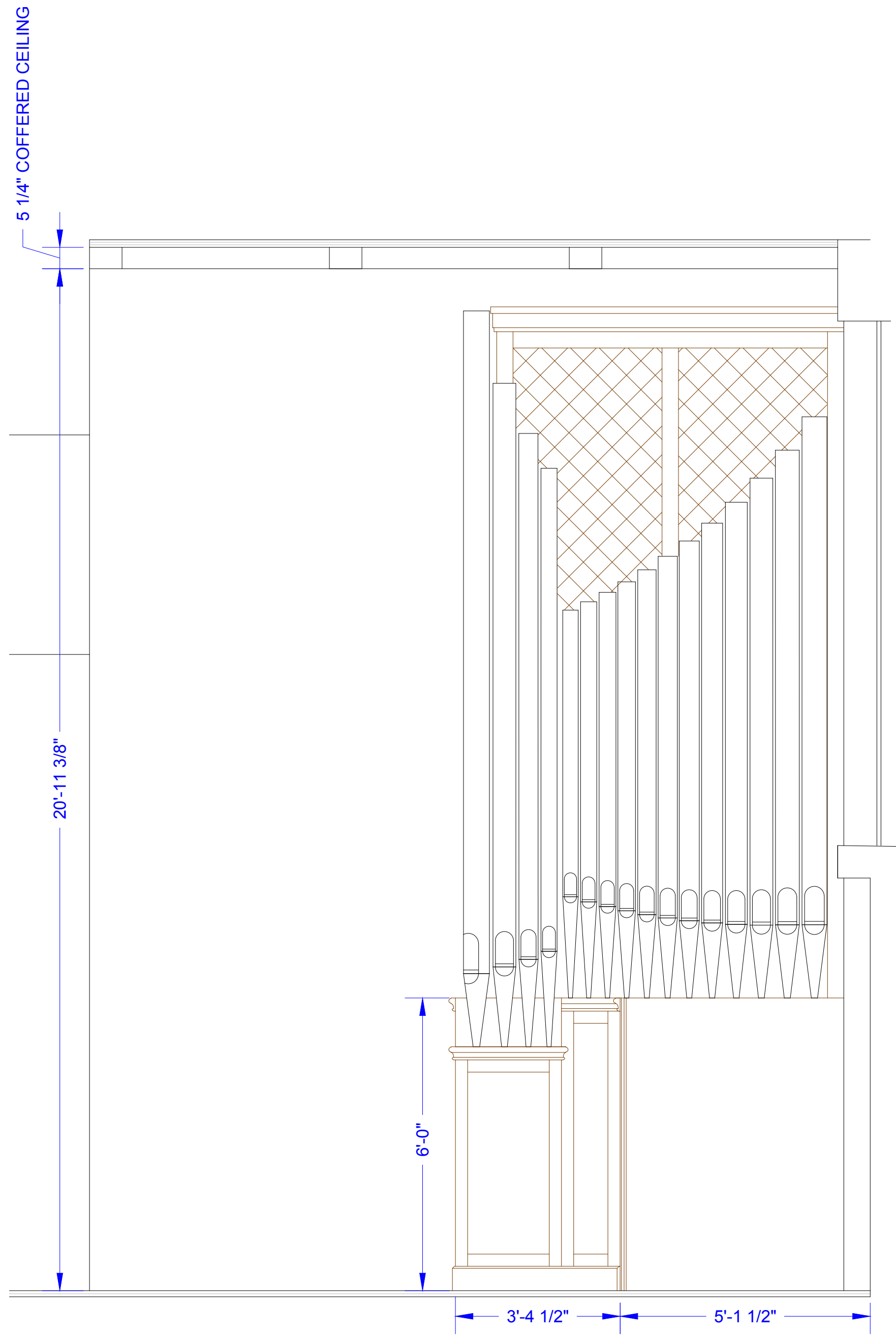
SECTION
