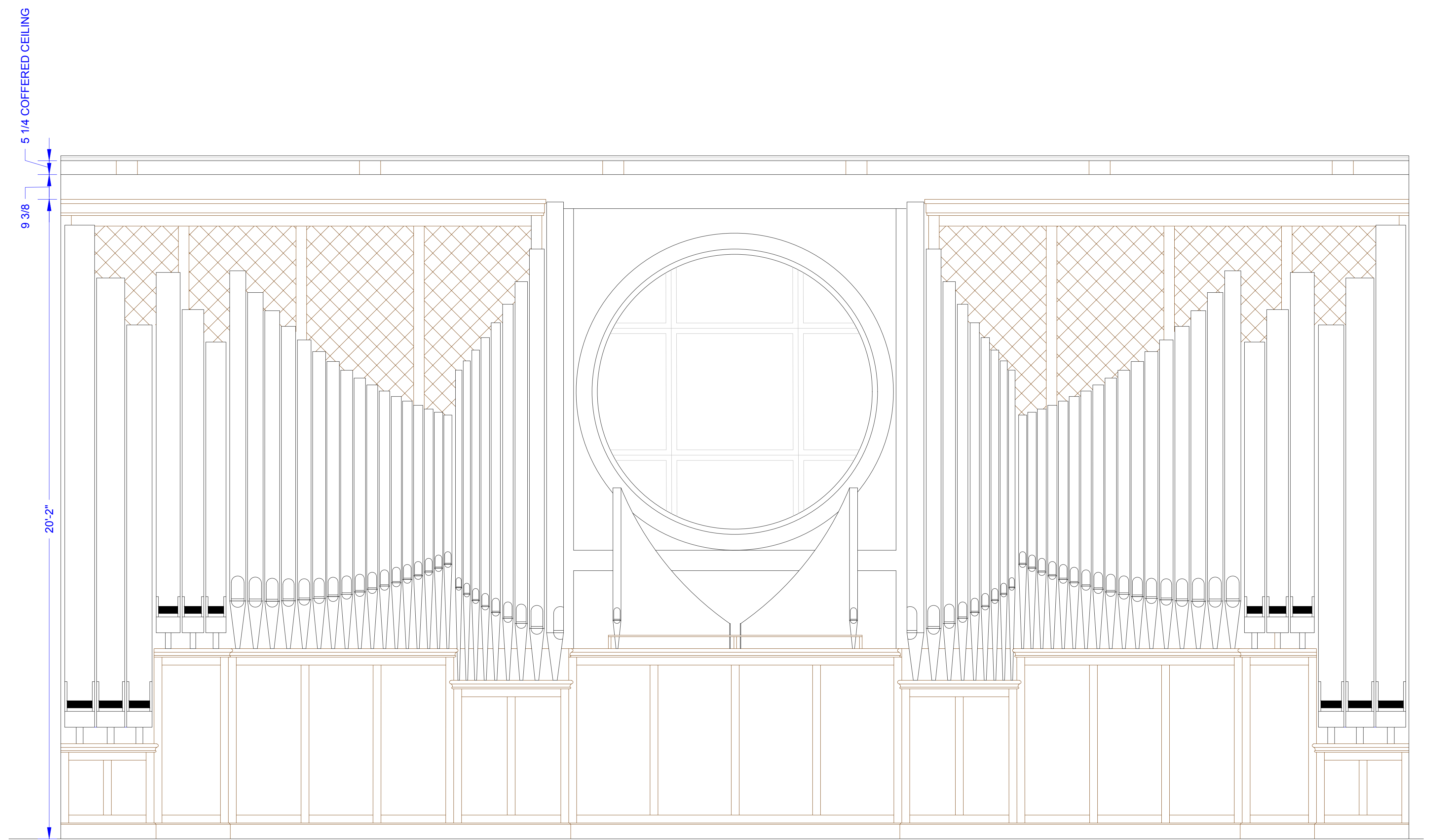
FRONT ELEVATION
